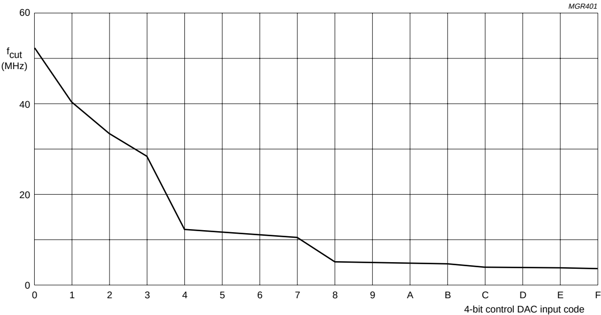
Fig.13 AGC bandwidth.
