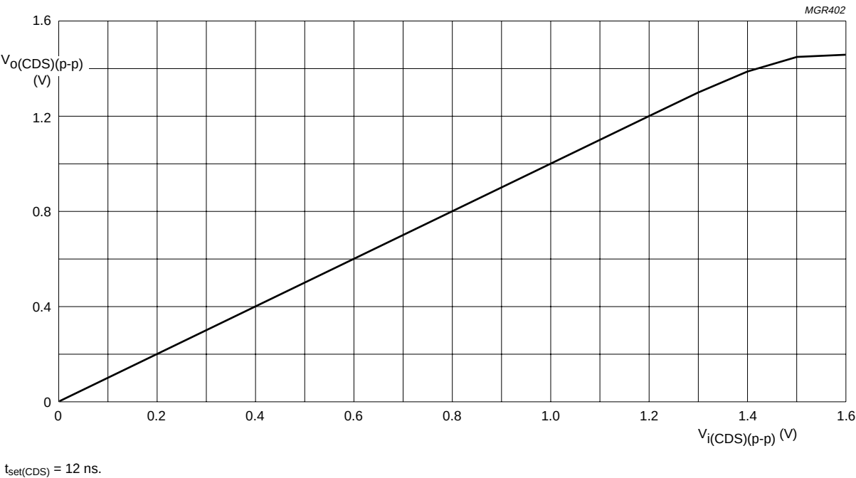
Fig.14 CDS output.
